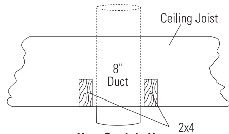
Vent Straight Up Through the Ceiling
