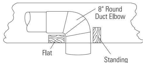
*Vent Between Ceiling Joists
